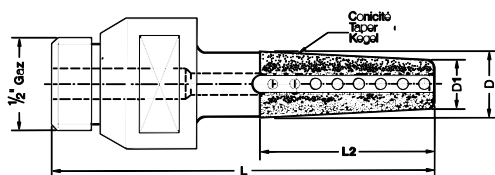
Male reamer – code T121
