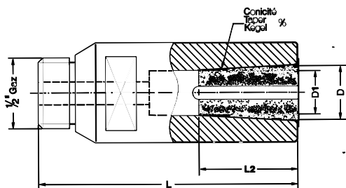
Female reamer – code T122
